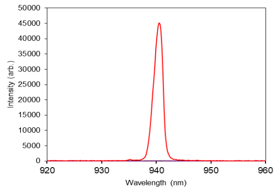
⊗ Spectral characteristics
